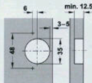
Drilling pattern 48/6
