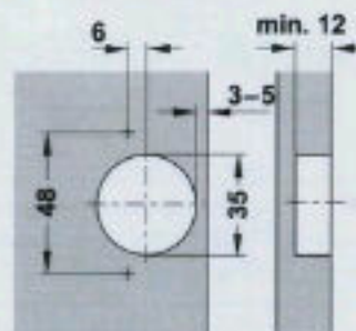
Drilling pattern 48/6
