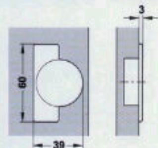
Drilling dimensions for cup fixing
