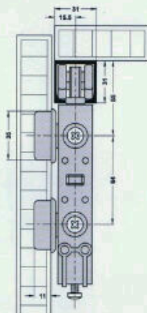
Top running gear, for outer door
